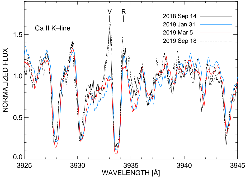
Figure 1. The chromospheric Ca II K-line, 3933\text{\AA} , from TRES echelle spectra, displays asymmetric emission wings [ marked as a V(violet) and R(red) feature ]. The appearance of V \leq R , signals wind absorption from a differentially expanding atmosphere in 2019 January and March. The profile lost this asymmetry in 2019 September, mimicing the earlier profile on 2018 September 14.
