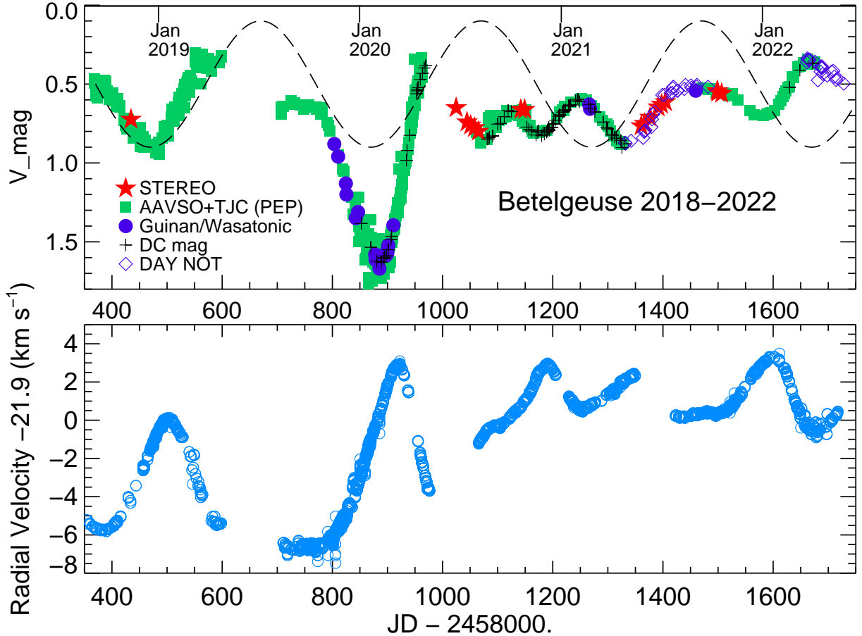
Figure 4. V-Magnitude ( upper panel ) from the AAVSO (2022), STEREO, the Wasatonic Observatory, D. Corona, and daytime measures (DAY NOT). The broken line marks a \sim 400 day period. This period is no longer present after the Great Dimming. Lower panel: Radial velocity of Betelgeuse from STELLA during 2018–2022.
