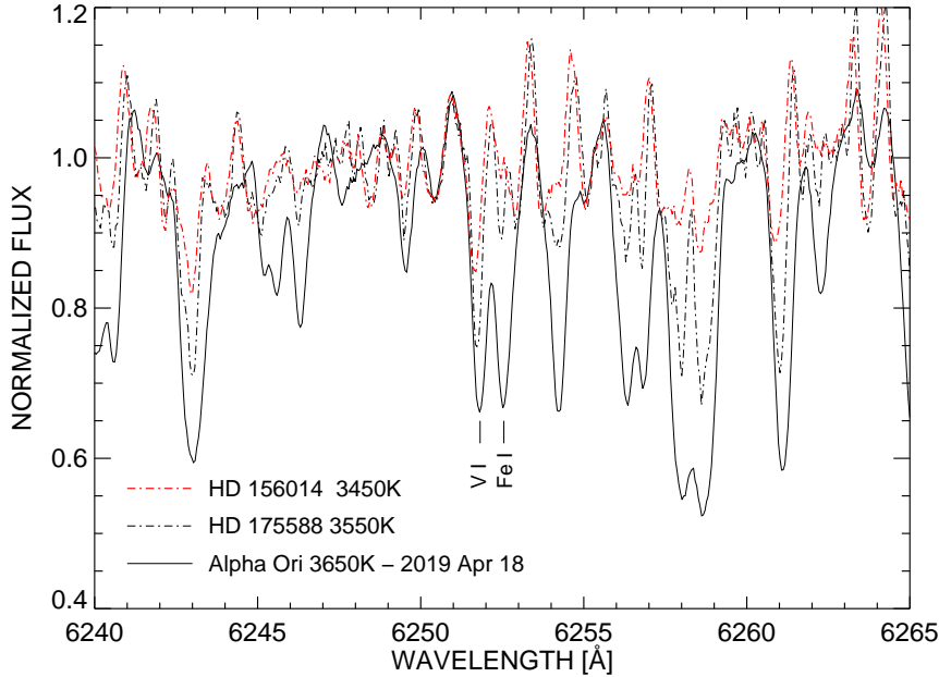
Figure 3. TRES spectra of Betelgeuse in 2019 April, a cooler supergiant (HD 156014), and a bright giant star (HD 175588). Note the systematic weakness of the absorption features as the effective temperature of the star decreases. At lower temperatures, the Fe I line at 6252.55\text{\AA} becomes blended with an unidentified absorption line. At the lowest temperature (3450K), the unidentified line dominates the Fe I line, making the ratio measurement (V I/Fe I) in Betelgeuse a lower limit when the star is faint.
